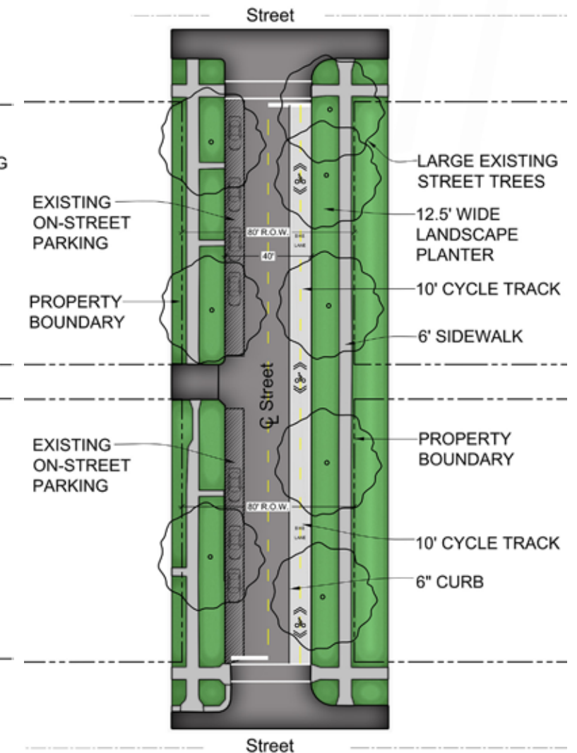
TYPICAL STREET WITH CYCLE TRACK
