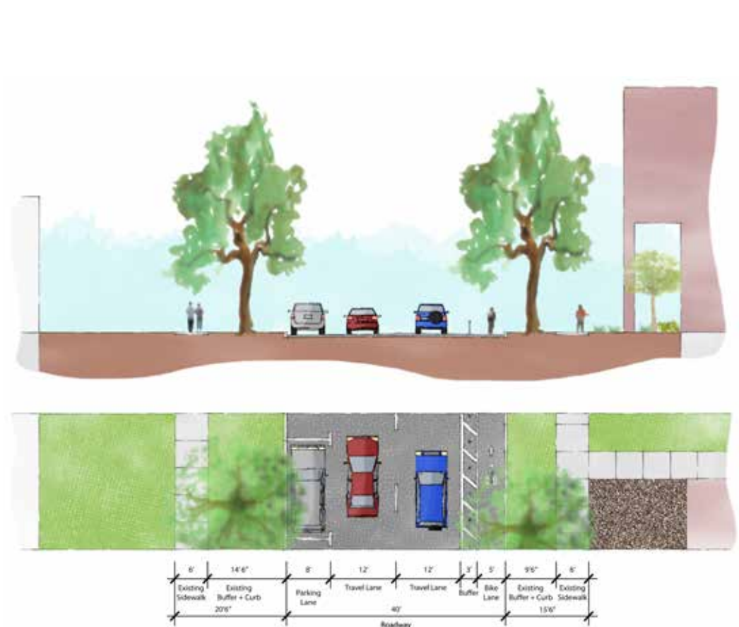
Possible future Idaho Street section after recommended improvements.
